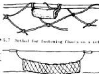
5.8 A scheme for floating gill nets.
