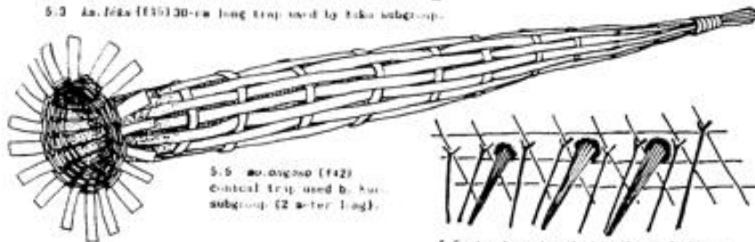
5.6 A scheme for tu.biya (F43) fishing.
